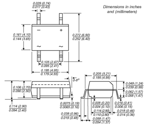
TO-269AA (MBS)
