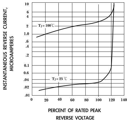
FIG. 3-TYPICAL REVERSE CHARACTERISTICS
