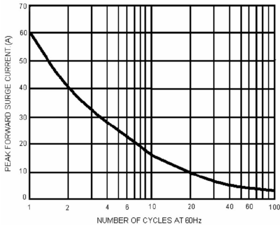
FIG.1-MAXIMUM NONO-REPETITIVE FORWARD SURGE CURRENT PER BRIDGE ELEMMENT
