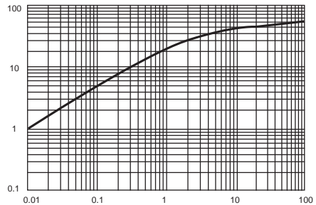
t, PULSE DURATION, sec.
