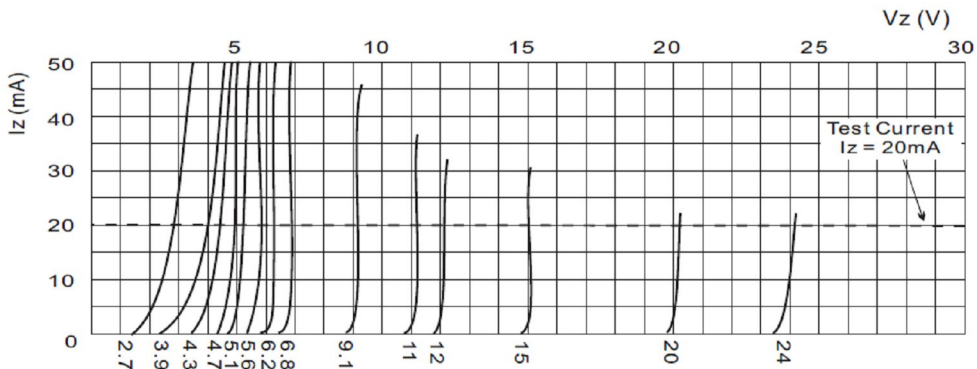
Fig.2 Break Characteristic
