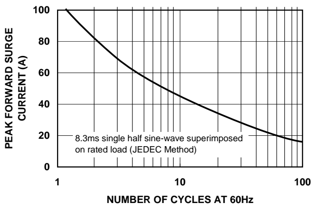
FIG.5.µ MAXIMUM NON-REPETITIVE PEAK FORWARD SURGE CURRENT
