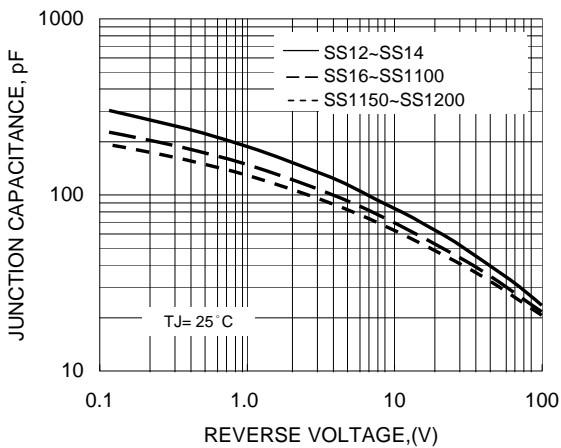
FIG. 5-TYPICAL JUNCTION CAPACITANCE
