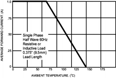
FIG.1- MAXIMUM TYPICAL FORWARD CURRENT DERATING CURVE
