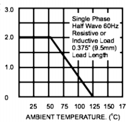
FIG.2- MAXIMUM AVERAGE FORWARD CURRENT DERATING
