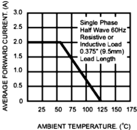
FIG.2- MAXIMUM AVERAGE FORWARD CURRENT DERATING
