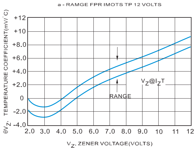
FIGURE 2 - TEMPERATURE COEFFICIENTS (-55° C TO +150° C TEMPERATURE RANGE; 90% OF THE UNITS ARE IN THE RANGES INDICATED.)
